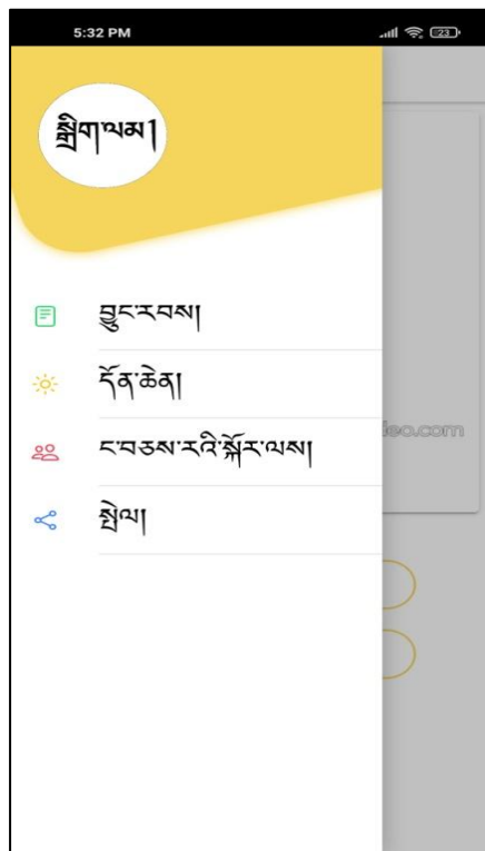
Fig. 8. Navigation Drawer
