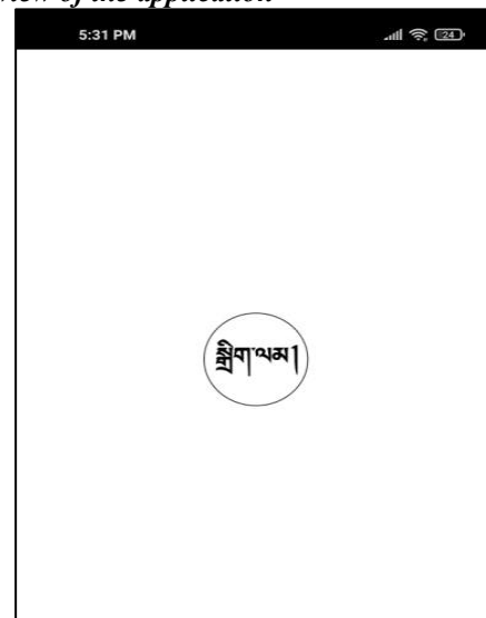
Fig. 6. Splash Screen
