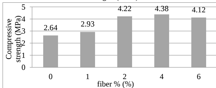
Figure 4: Compressive strength Vs fiber percentage
