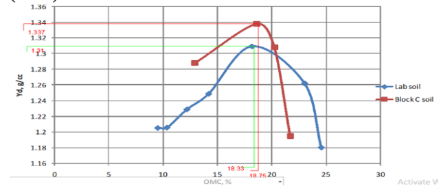
Figure 2: Comparative MDD and OMC of two soil samples
