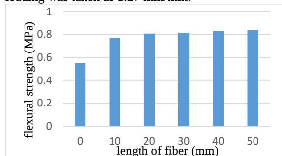
Figure 3: Graph of flexural strength Vs length of fiber
