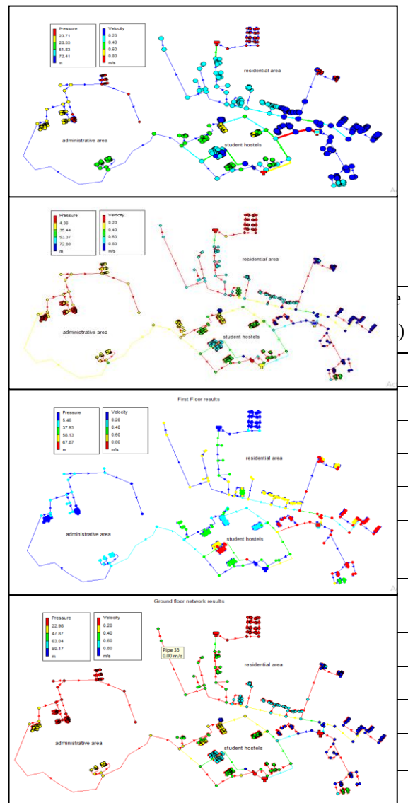
Figure 5: Floor-wise EPANET results
