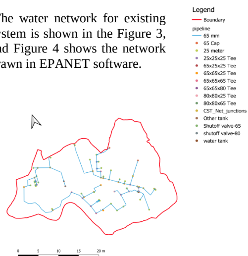
Figure 3: CST Water Distribution Network
