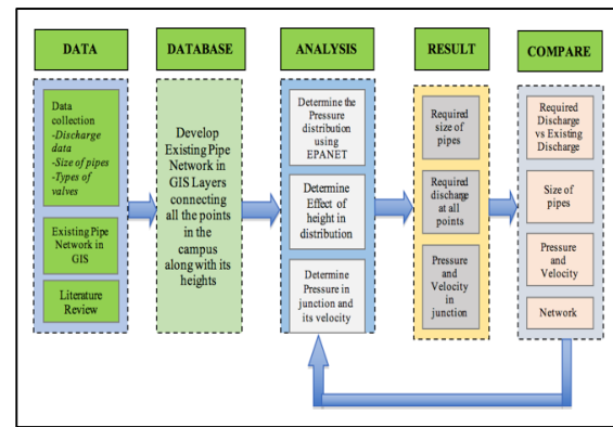
Figure 2: Methodology Flowchart
