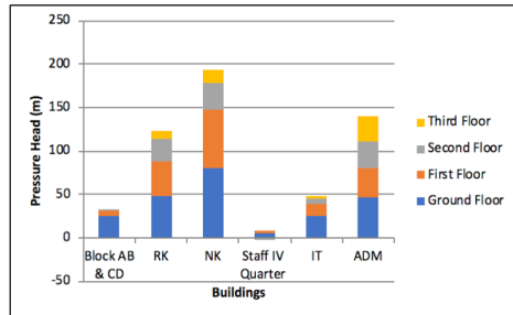
Figure 6: A graph showing the relation between pressures and building height
